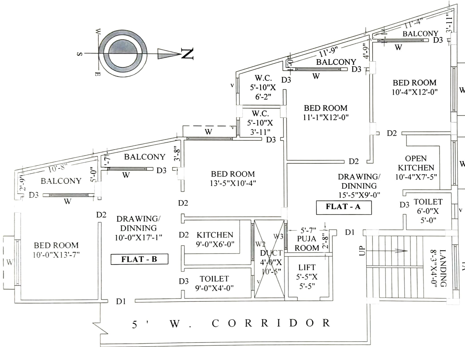
1ST TO 5TH FLOOR PLAN FLAT - A & FLAT - B SCALE - 1:96
