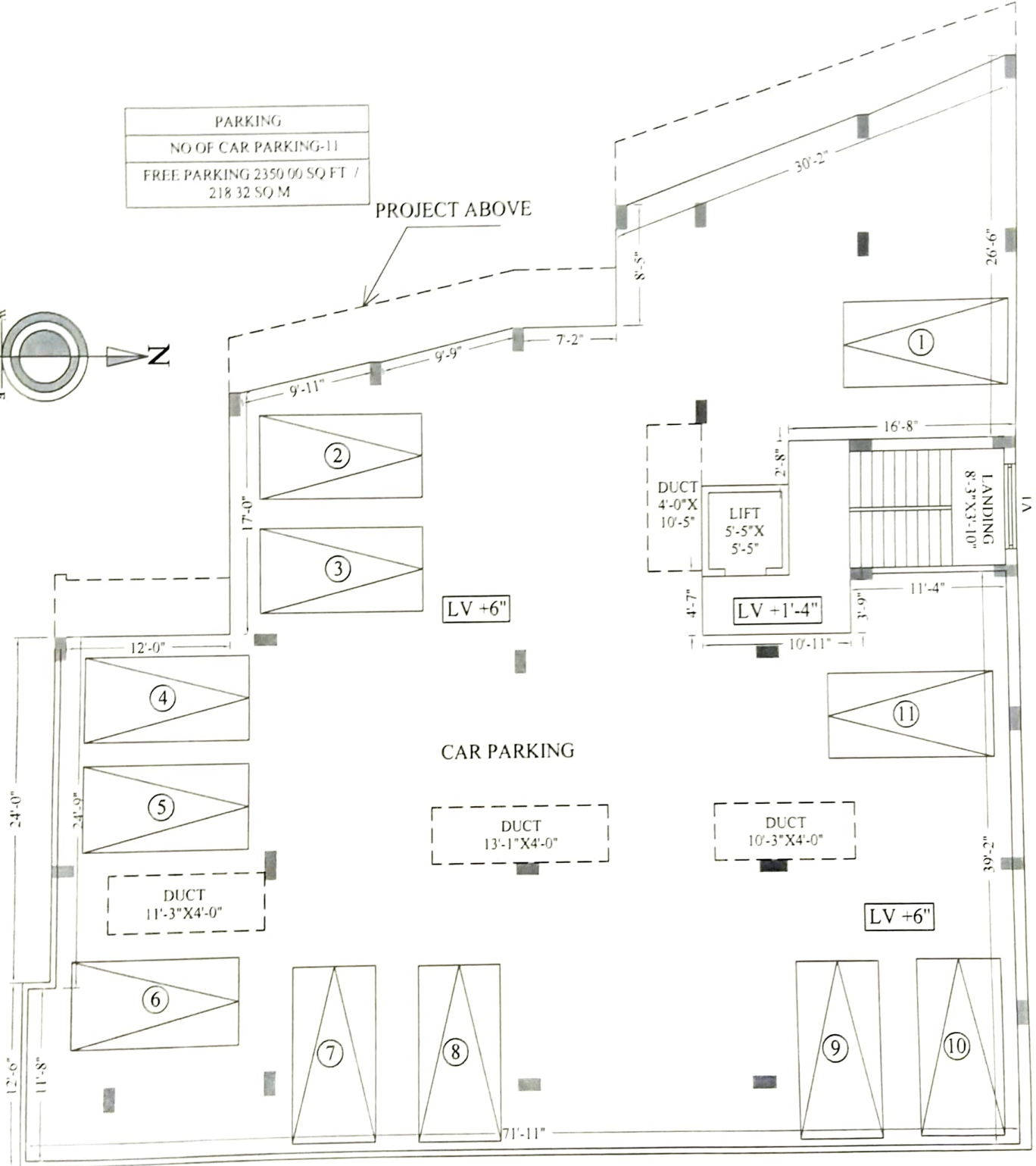
GROUND FLOOR PLAN SCALE - 1:96
