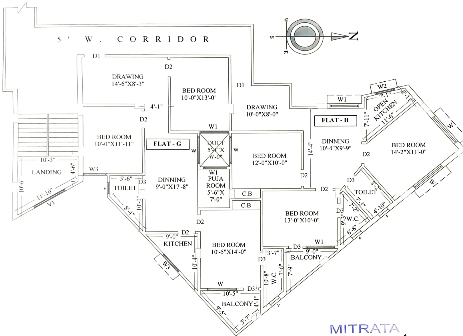
2ND TO 5TH FLOOR PLAN FLAT - G & FLAT - H SCALE - 1:96
