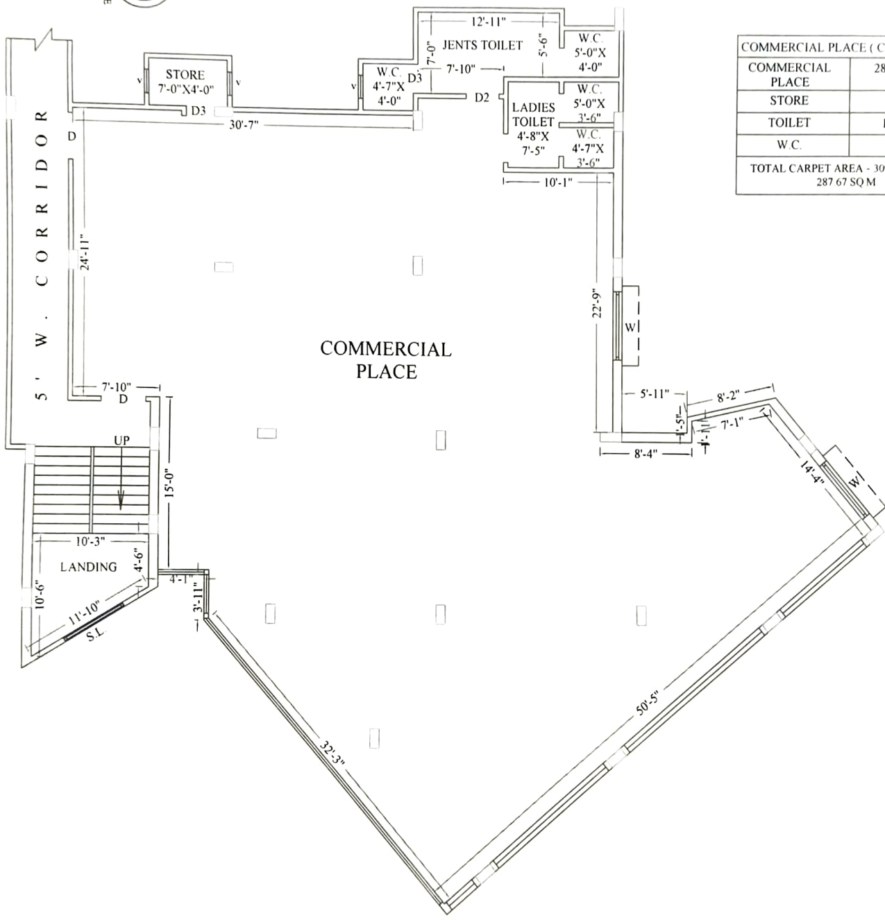
1ST FLOOR PLAN COMMERCIAL PLACE SCALE - 1:96
